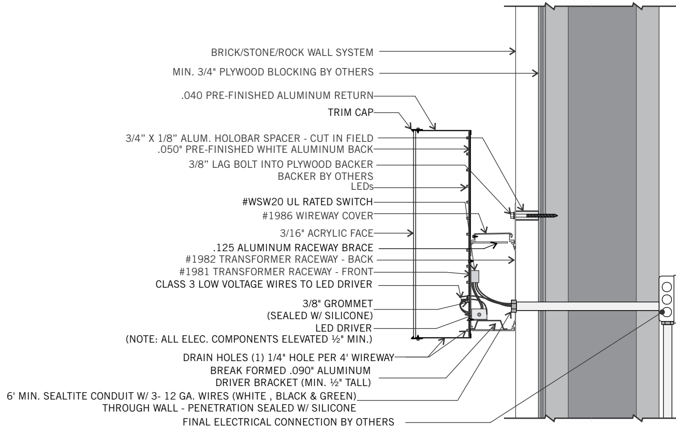
2 CROSS SECTION SCALE: NTS
