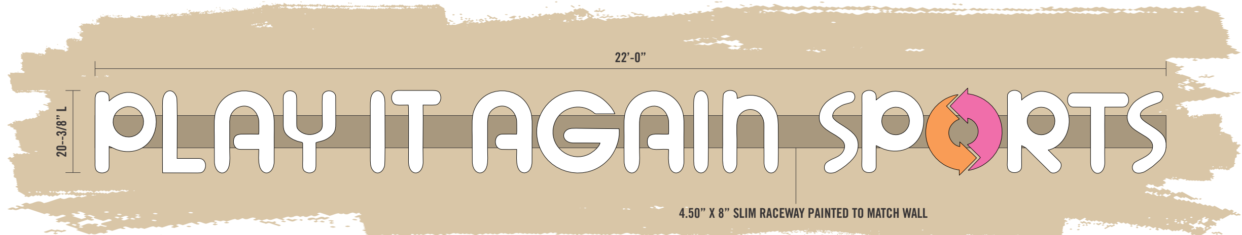
1 ILLUMINATED WALL SIGN SCALE: 1/2"=1'-0"
